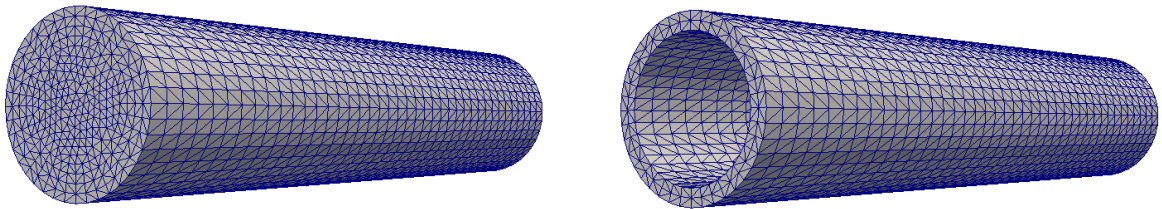
FIGURE 21 - Refinement of the full fluid mesh and the fluid part of the thin predictor
