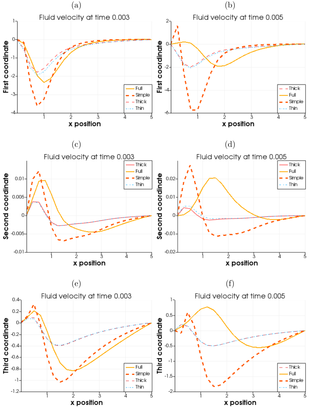
FIGURE 26 - Plots of the fluid's velocity on the line, with \Delta t = 10^{-3}
