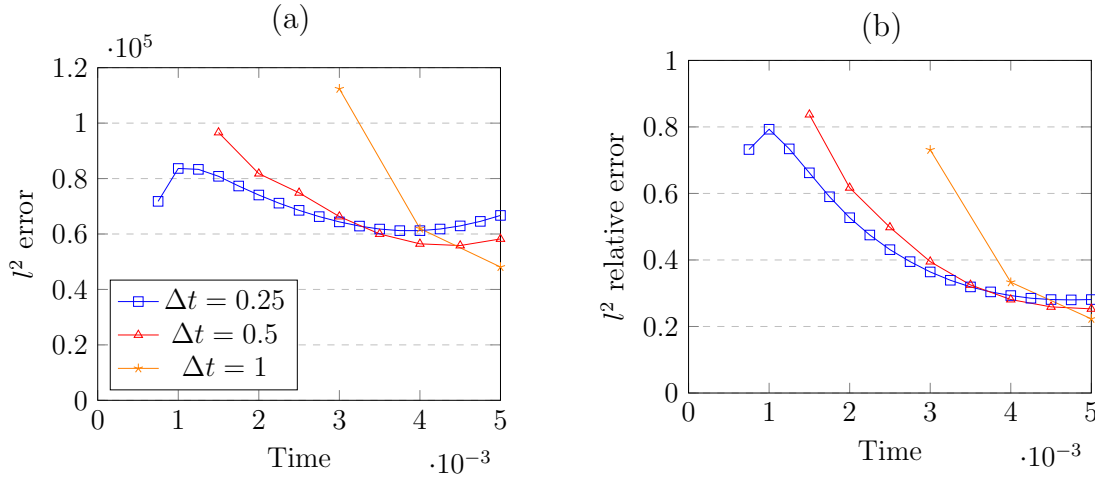
FIGURE 10 - Errors for the fluid pressure using the thick predictor
