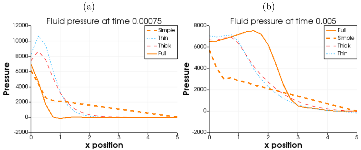
FIGURE 15 - Plots of the fluid's pressure on the line, with \Delta t = 0.25 \times 10^{-3}
